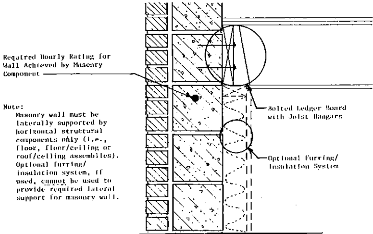
FIGURE 3 Multi-Wythe Masonry Wall (Bearing Condition)
