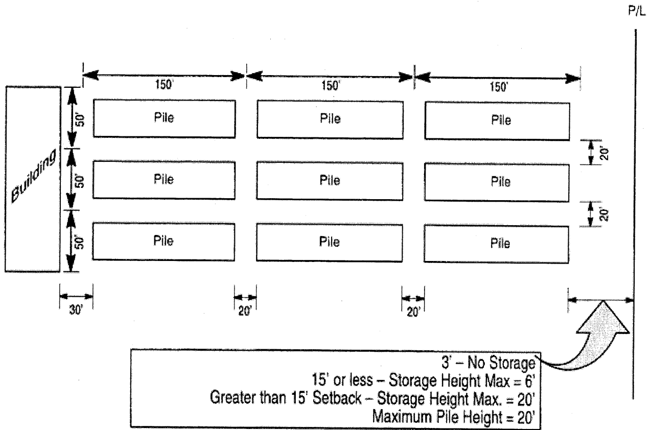
A-14.10 (2) OUTSIDE STORAGE SCHEMATIC.
