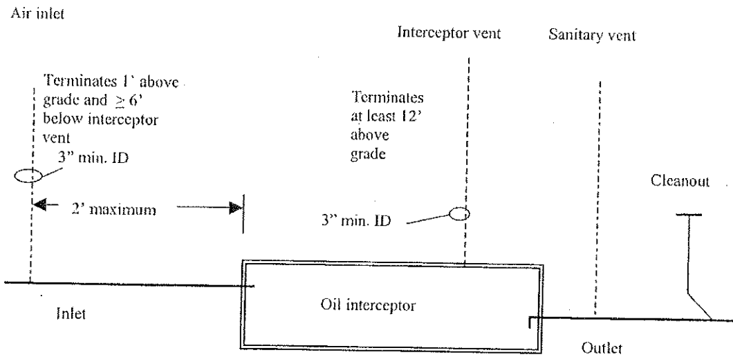
VENTS AS SHOWN MUST TERMINATE INDEPENDENTLY.
