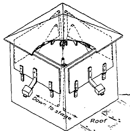
VIEW OF WOODEN VENTILATOR
