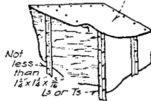
Typical Construction METAL OR ASBESTOS
