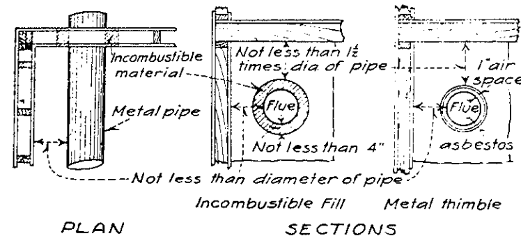
PLAN SECTIONS
