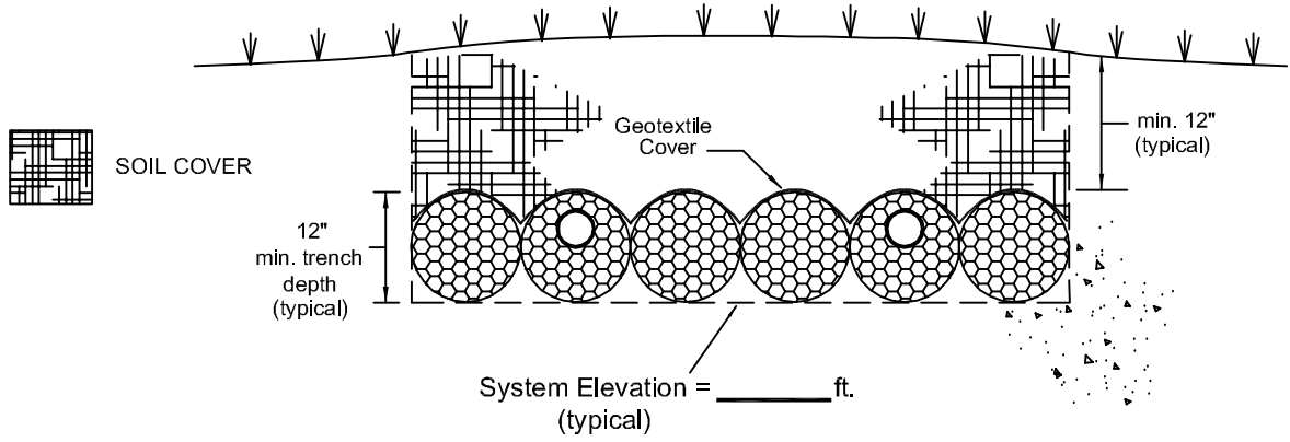
TYPICAL TRENCH CROSS SECTION VIEW (No Scale)
