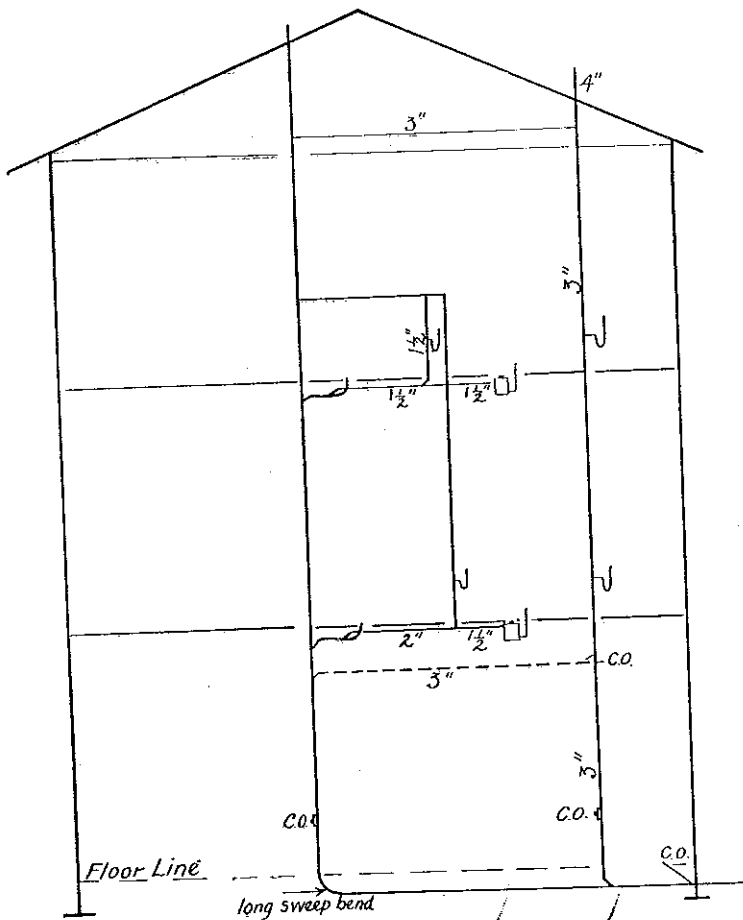
(5) Illustrating permissible method of bathroom and sink waste and vent installation. H 62.06 (1), H 62.07 (8).
