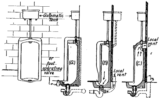
(31) Showing individual urinal set into the floor. H 62.09 (2), H 62.12 (9).
