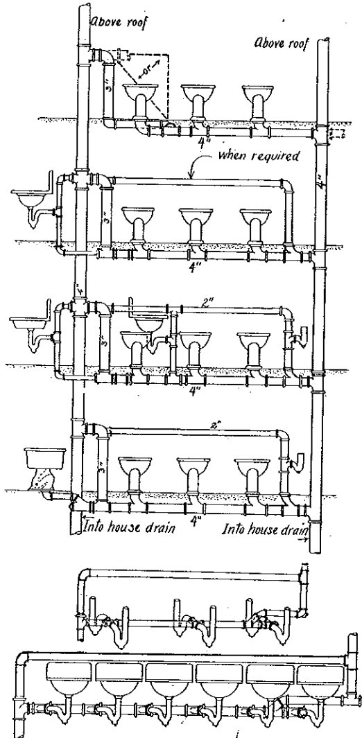
(11) Illustrating method of circuit or continuous venting. H 62.03 (1), (3); H 62.06 (5); H 62.07 (2) (b), (c); H 62.08 (d).
