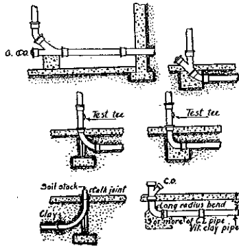
(9) Showing methods of supporting soil pipe stacks at their base. H 62.06 (3), (6)
