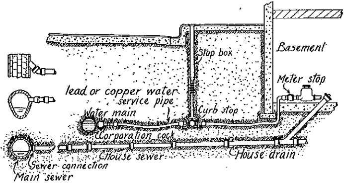
(3) Typical installation of house drain to point within building. H 62.05 V(1).
