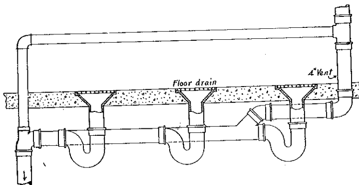
(24) Showing circuit waste and vent method of floor drain installation. H 62.07 (2) (b), H 62.10 (2).
