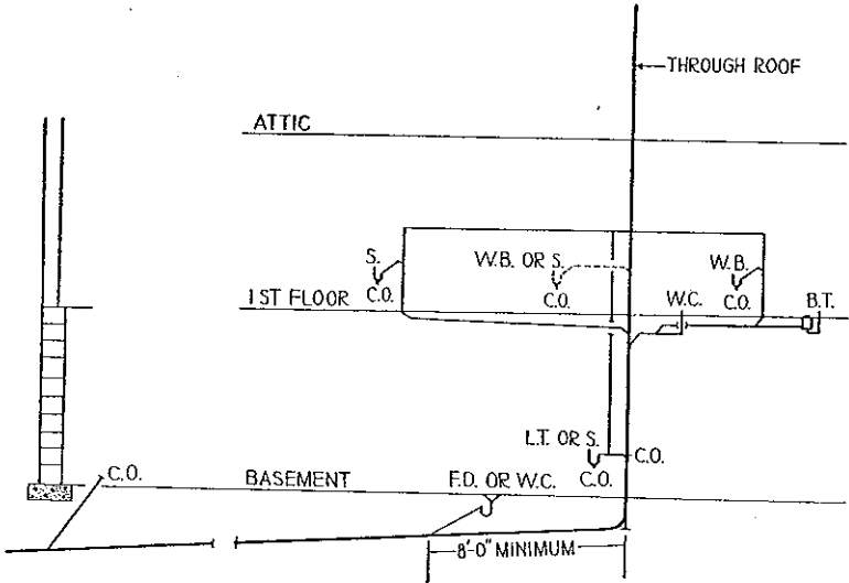
(6) Illustrating minimum requirements for typical one-story building installation. H 62.06 (1), H 62.07 (6), (7) (b).
