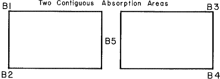
Example Of Soil Boring Locations For Two Contiguous Absorption Areas
