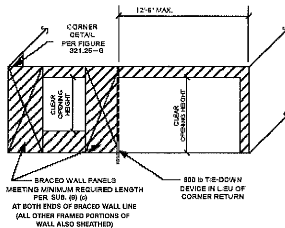
FIGURE 321.25-J CONTINUOUSLY SHEATHED BRACED WALL LINE — FIRST BRACED WALL PANEL AWAY FROM END OF WALL LINE WITH TIE DOWN
