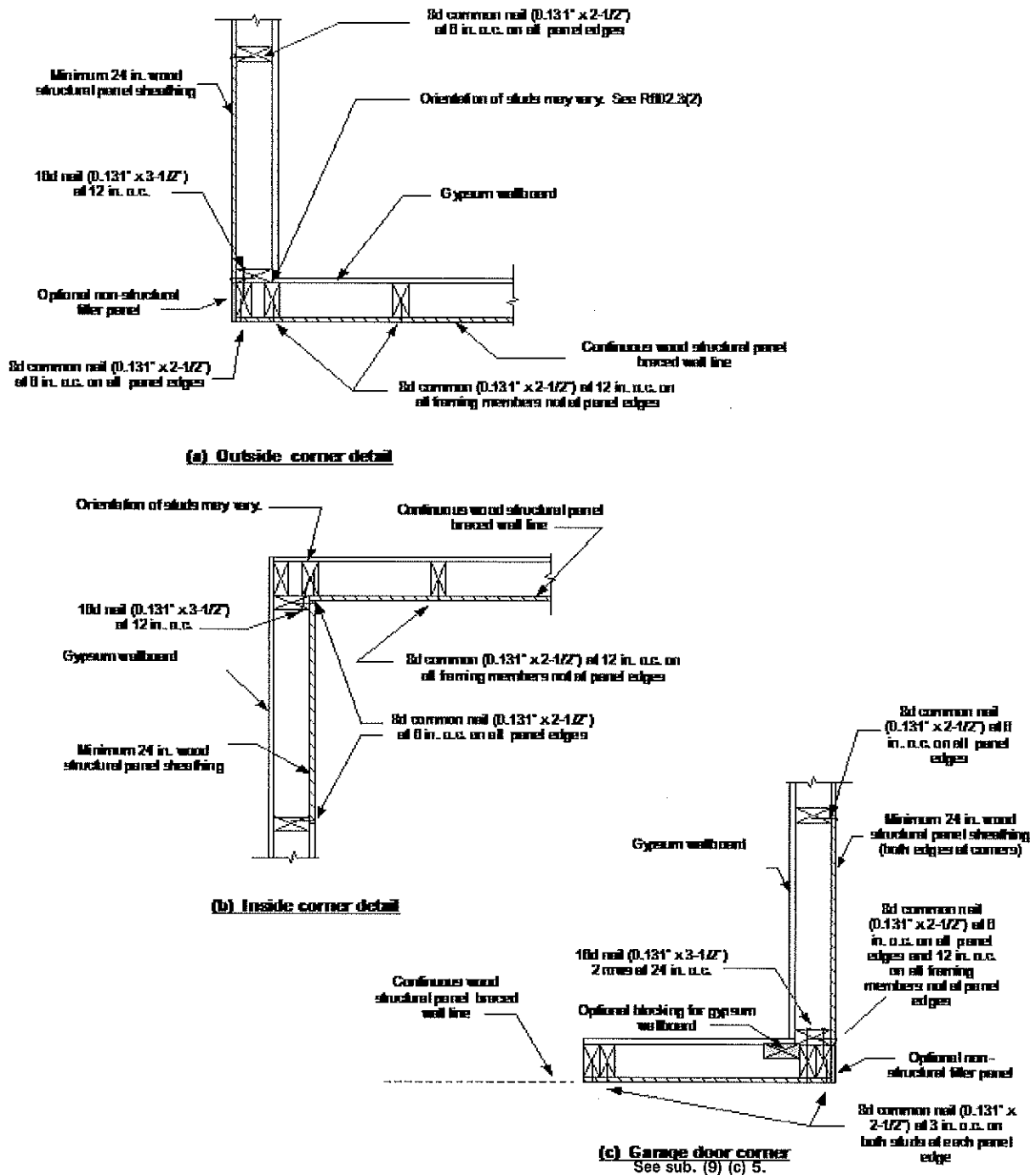
FIGURE 321.25-G TYPICAL EXTERIOR CORNER FRAMING FOR CONTINUOUS STRUCTURAL PANEL SHEATHING SHOWING REQUIRED STUD-TO-STUD NAILING
