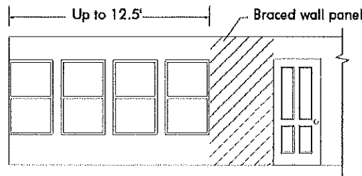
FIGURE 321.25-B PERMITTED BRACED WALL PANEL DISTANCES FROM ENDS OF A BRACED WALL LINE
