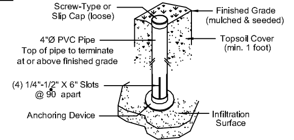
OBSERVATION PIPE DETAIL (No Scale)
