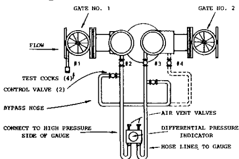
TESTING DIAGRAM
