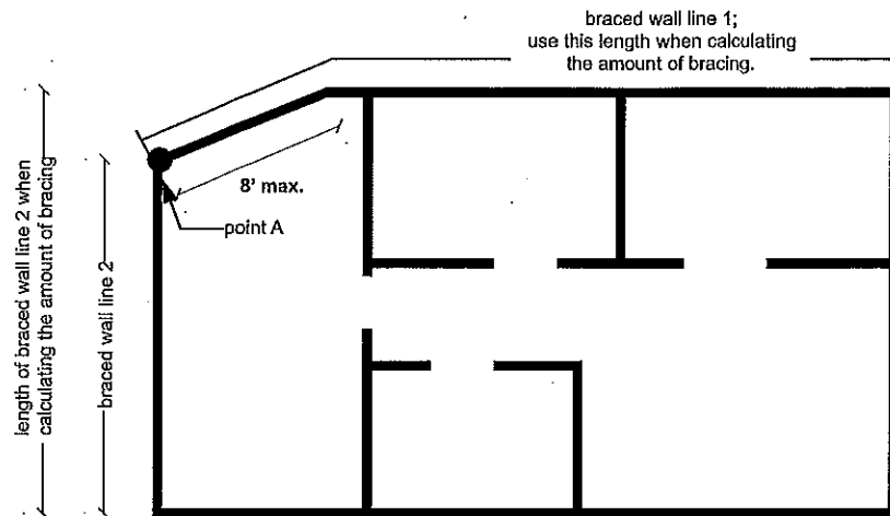
FIGURE 21.25-D ANGLED CORNERS
