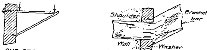
DETAIL OF WALL BEARING
