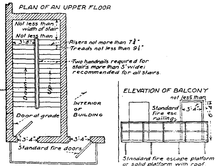
EXTERIOR ENCLOSED STAIR
