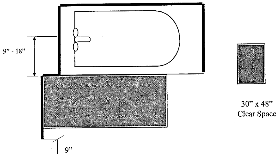
FIGURE 57.871-2 CLEAR FLOOR SPACE/CENTERED CONTROLS
