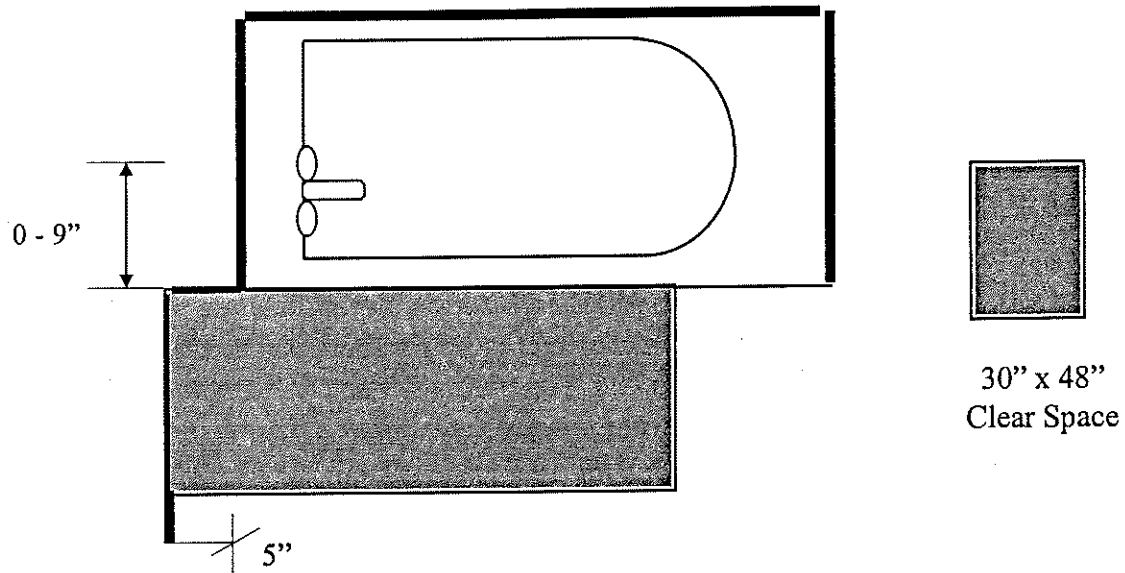
FIGURE 57.871-1 CLEAR FLOOR SPACE/OFFSET CONTROLS
