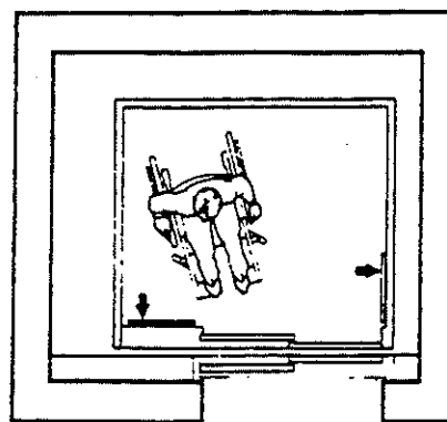
(d) Alternate Locations of Panel with Side Opening Door
