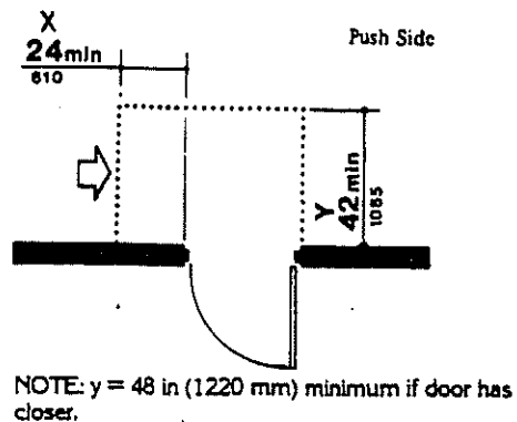
(c) Latch Side Approaches — Swinging Doors
