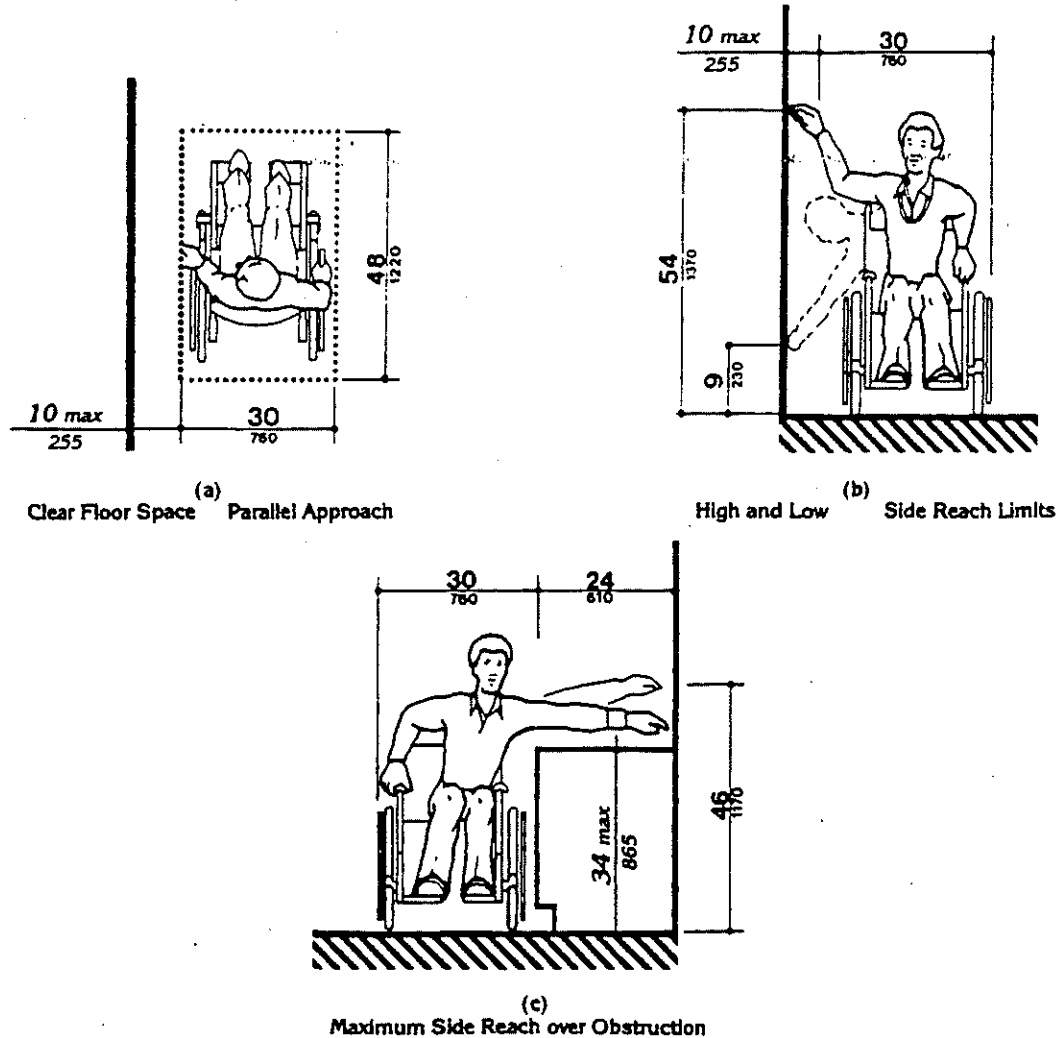
Fig. 6 Side Reach
