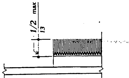
Fig. 8 (f) Carpet Pile Thickness
