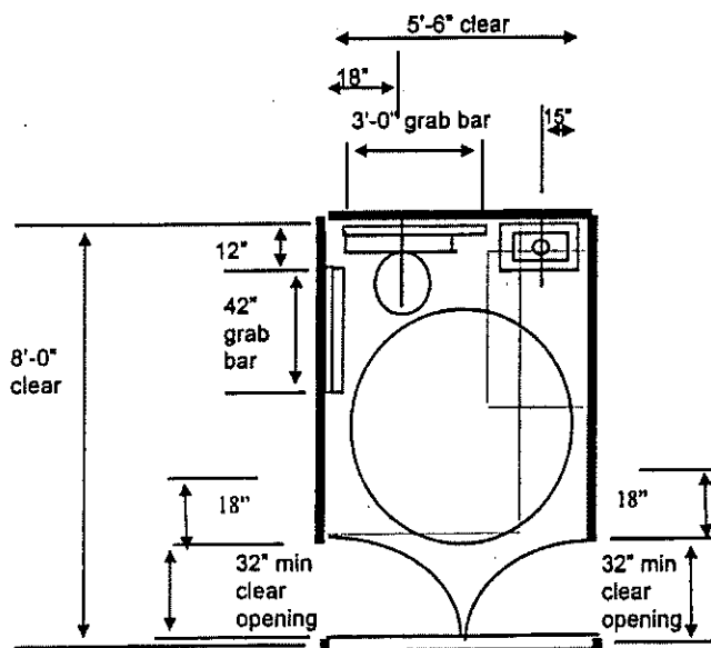
Figure 69.35-5/Toilet Room
