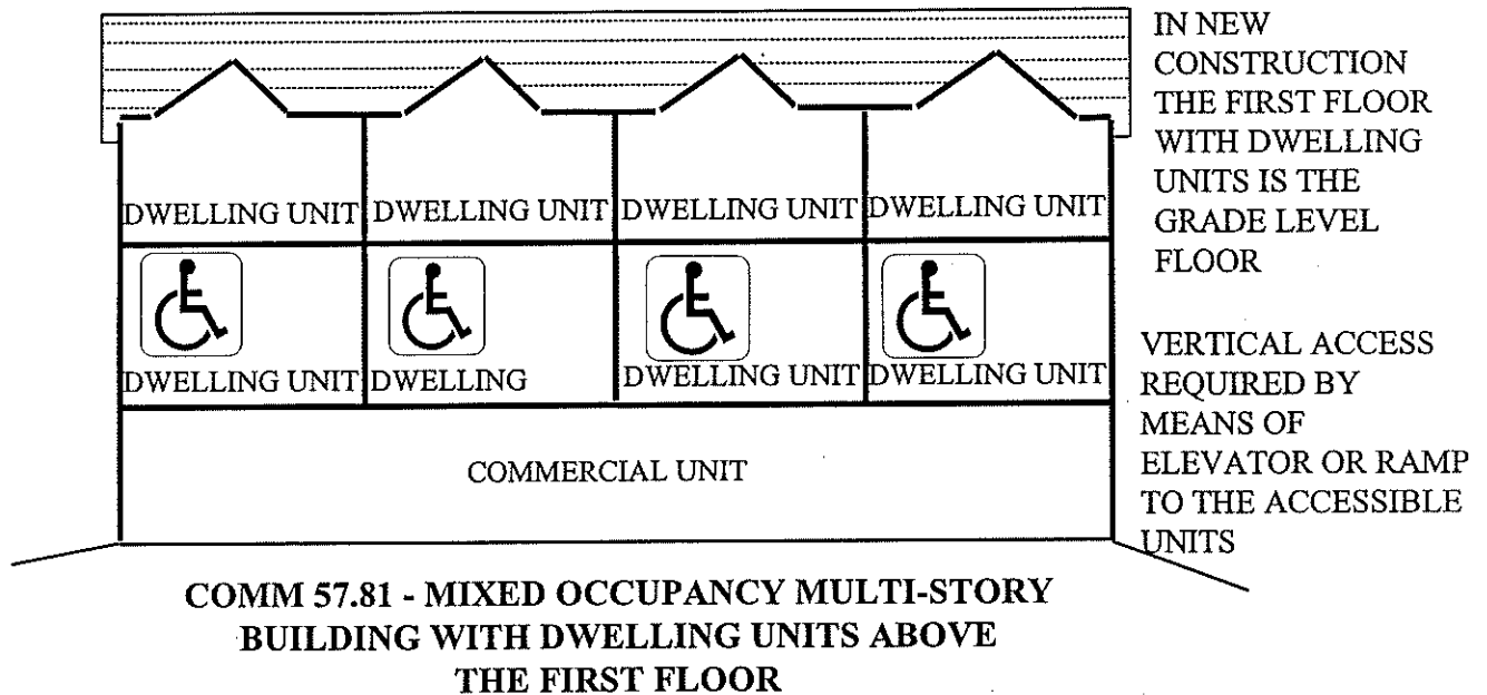
COMM 57.81 - BUILDING WITH ELEVATOR
