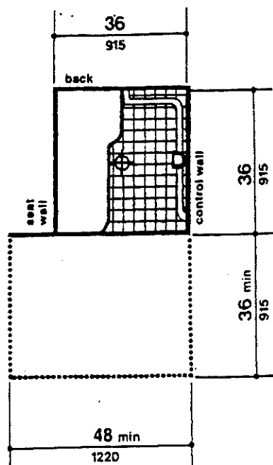
(a) 36-in by 36-in (915-mm by 915-mm) Stall
