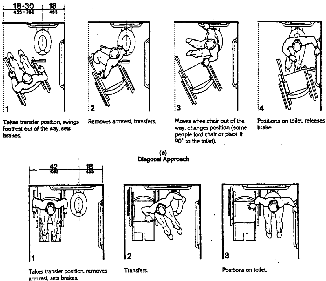
Fig. A6 Wheelchair Transfers
