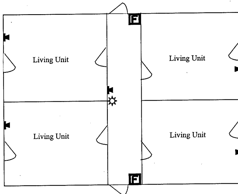
Living Units Not Stacked or Living Units With Common Required Exits per 66.34(1)(a)1.
