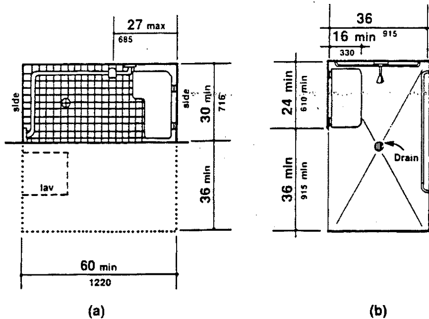
Fig. 57 Roll-in Shower with Folding Seat
