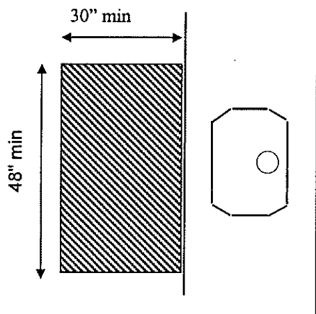
Lavatory Without Knee Space
