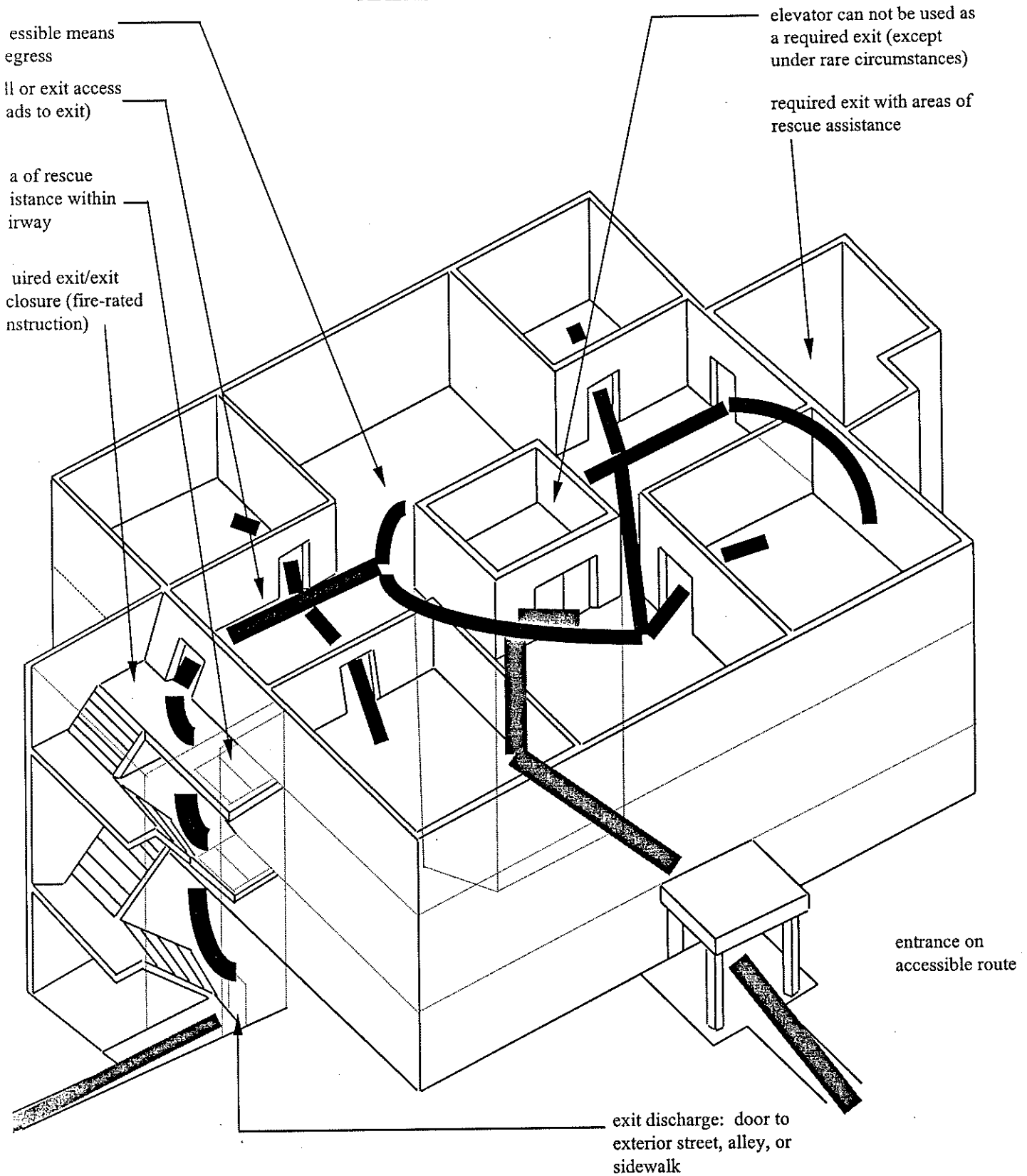
FIGURE 2 AREAS OF RESCUE ASSISTANCE
