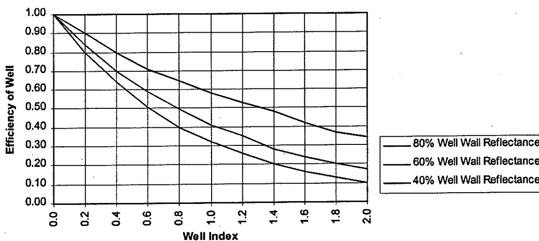
Figure 63.02 Well Efficiency
