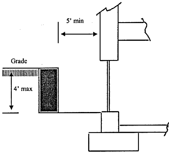
SECTION AT AREAWAY
