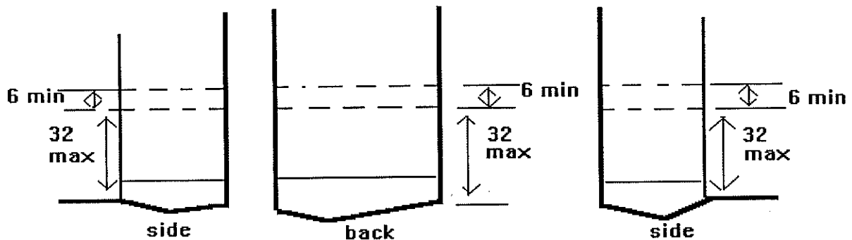
FIGURE 57.86-3 LOCATION OF GRAB BAR REINFORCEMENTS FOR ADAPTABLE SHOWERS
