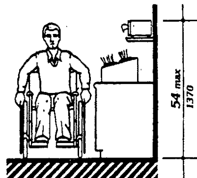
Fig. 54 Tableware Areas
