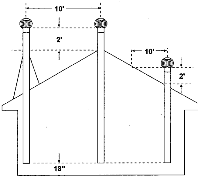
VENTILATION DUCTS, COMM 64.39
