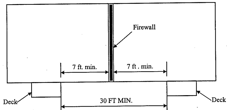
UNLIMITED OPENINGS COLUMN SUPPORTED DECKS
