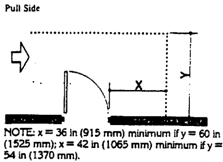
(a) Front Approaches — Swinging Doors
