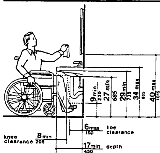
Fig. 31 Lavatory Clearances
