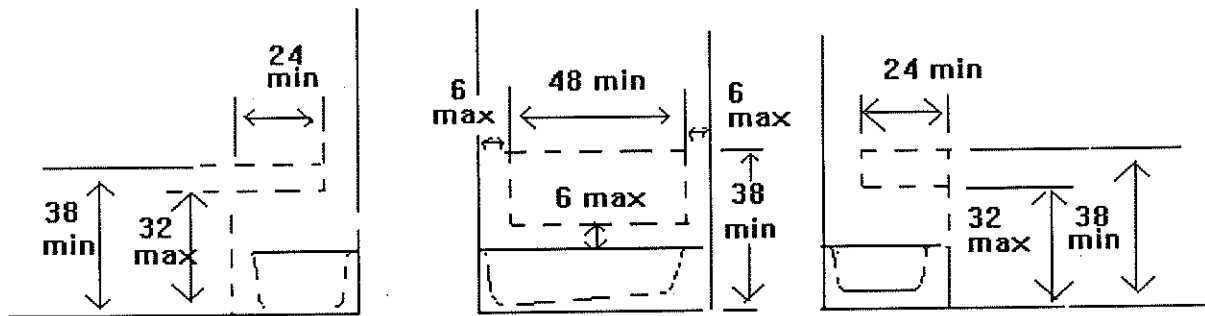
FIGURE 57.86-2 LOCATION OF GRAB BAR REINFORCEMENT FOR ADAPTABLE BATHTUBS
