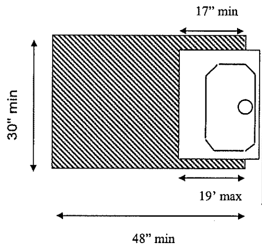
Lavatory With Knee Space
