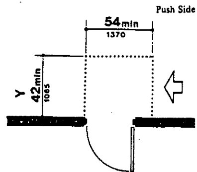
(b) Hinge Side Approaches — Swinging Doors
