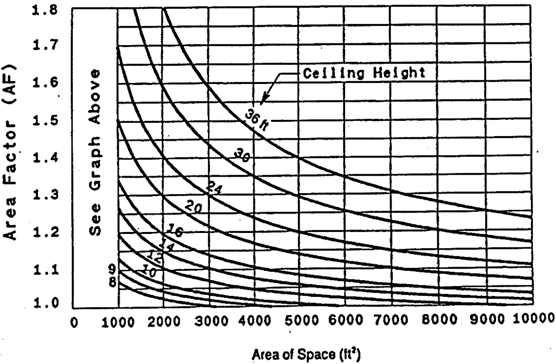
Figure 63.49 Area Factor
