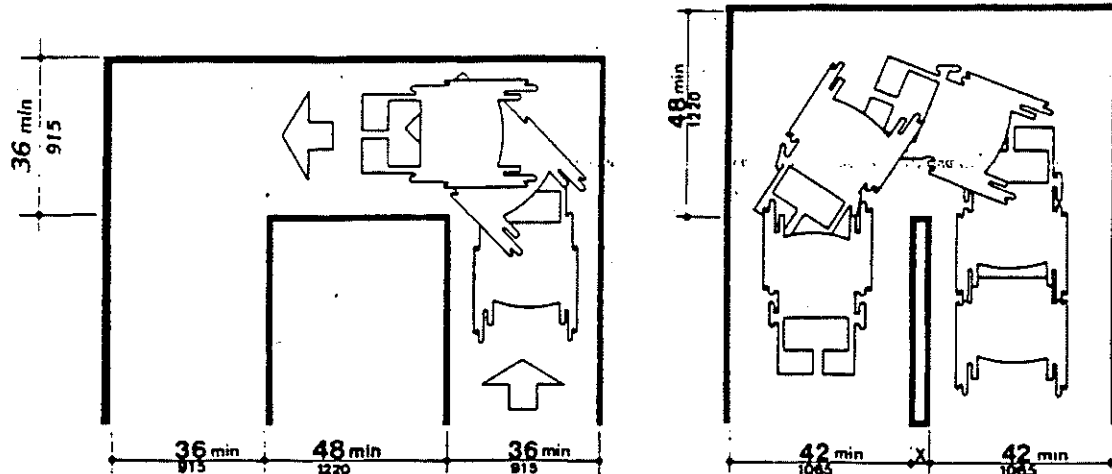
(a) 90° Turn
