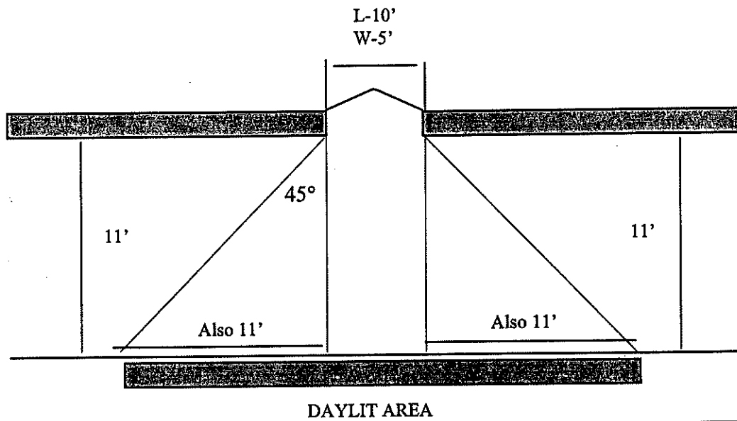
Figure A63.05-B Skylight Daylit Area
