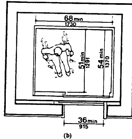
Fig. 22 Minimum Dimensions of Elevator Cars
