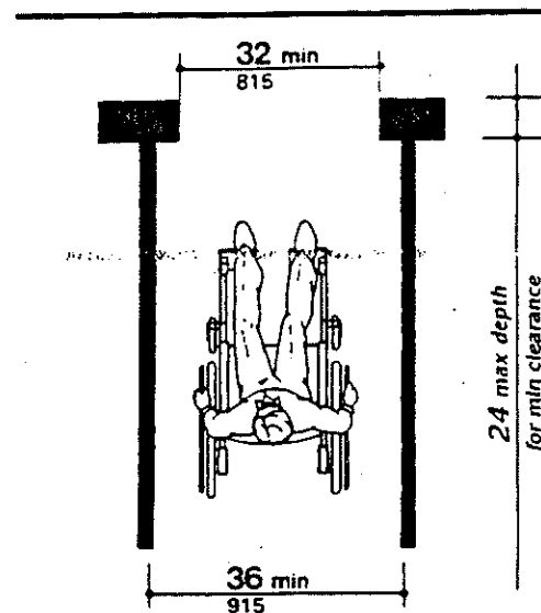
Fig. 1 Minimum Clear Width for Single Wheelchair
