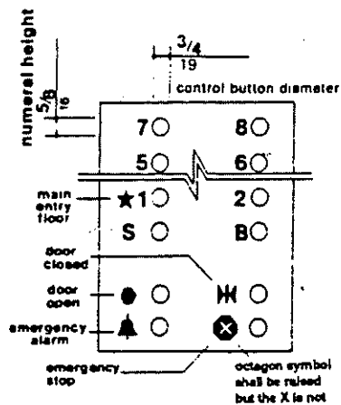
(a) Panel Detail
