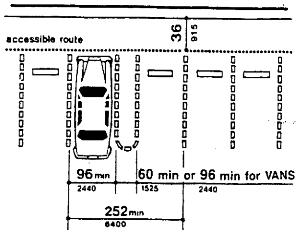
Fig. 9 Dimensions of Parking Spaces
