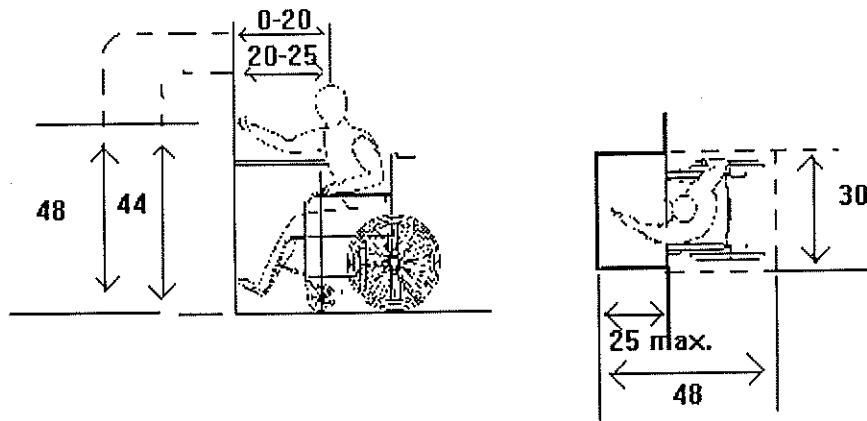
(b) Maximum Forward Reach Over an Obstruction
