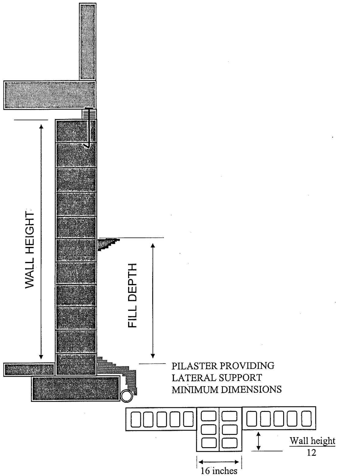
MASONRY WALLS BELOW GRADE COMM 53.322 (2)(d)
