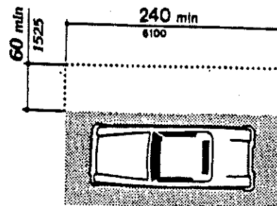
Fig. 10 Access Aisle at Passenger Loading Zones
