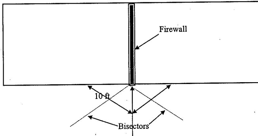
FIREWALL EXTENSION
