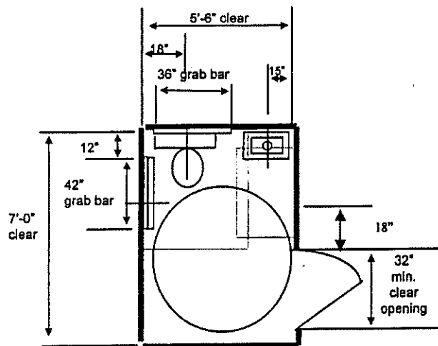
Figure 69.35-3/Toilet Room
