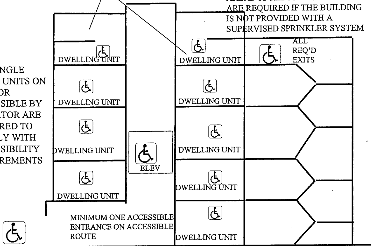
COMM 57.81 - BUILDING WITH ELEVATOR
