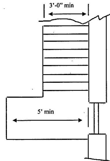
PLAN VIEW AT EXTERIOR STAIRWAY
