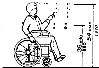
(b) Car Control Height
