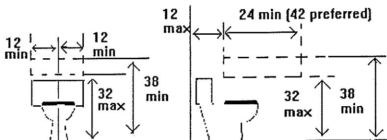
Reinforced Areas for Installation of Grab Bars
