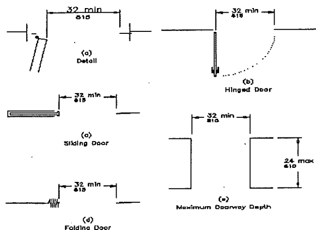
FIG. 24 Clear Doorway Width and Depth
