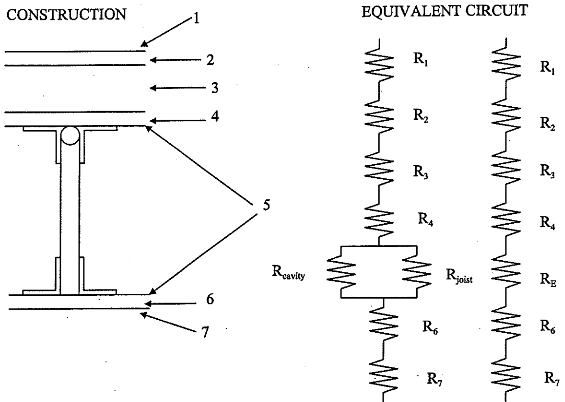
Figure 63.18-2 Calculation Procedure for Thermal Resistance of a Typical Roof Assembly
