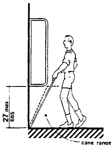
Fig. 8 (b) Walking Perpendicular to a Wall
