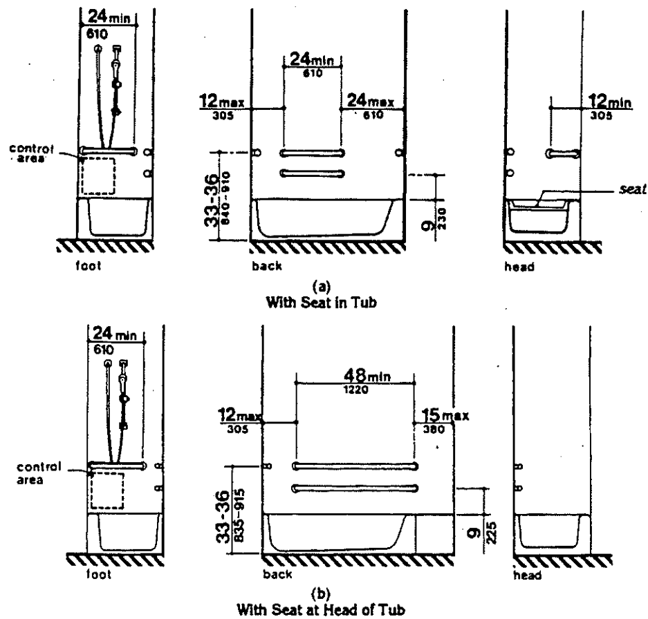
Fig. 34 Grab Bars at Bathtubs
