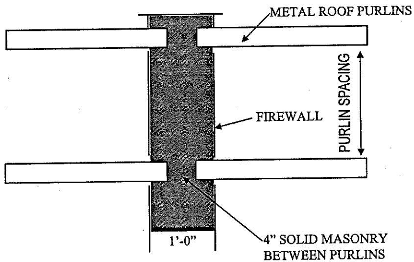
PLAN AT FIRE WALL
