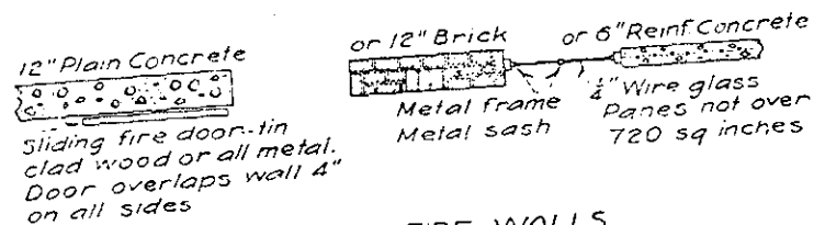
STANDARD FIRE WALLS
