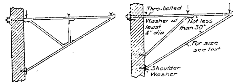
TWO TYPES OF TWO STAIR SUPPORT
