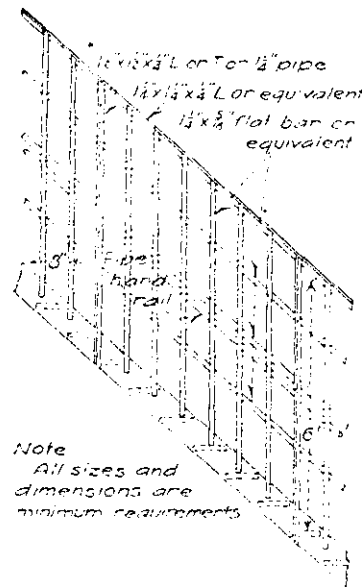
RAILING FOR HIGH BUILDINGS
