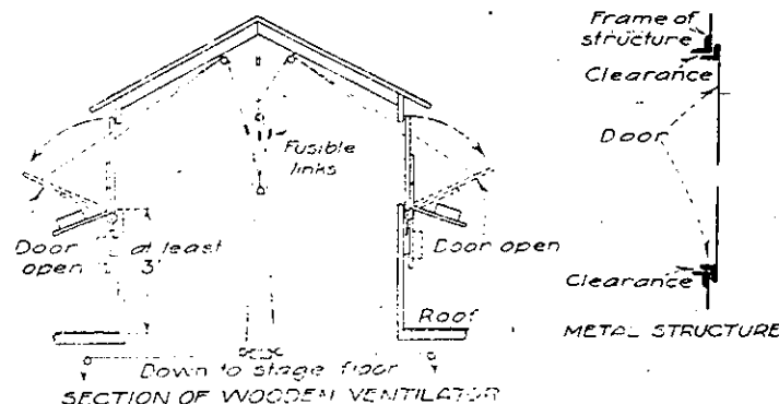
SECTION OF WOODEN VENTILATOR AUTOMATIC STAGE VENTILATOR
