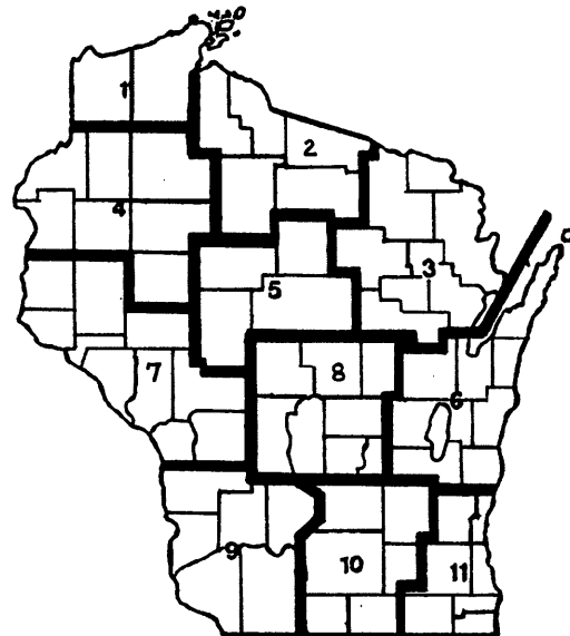
FIGURE 67.06 HEATING DEGREE DAYS PER YEAR - BASE 65°F
