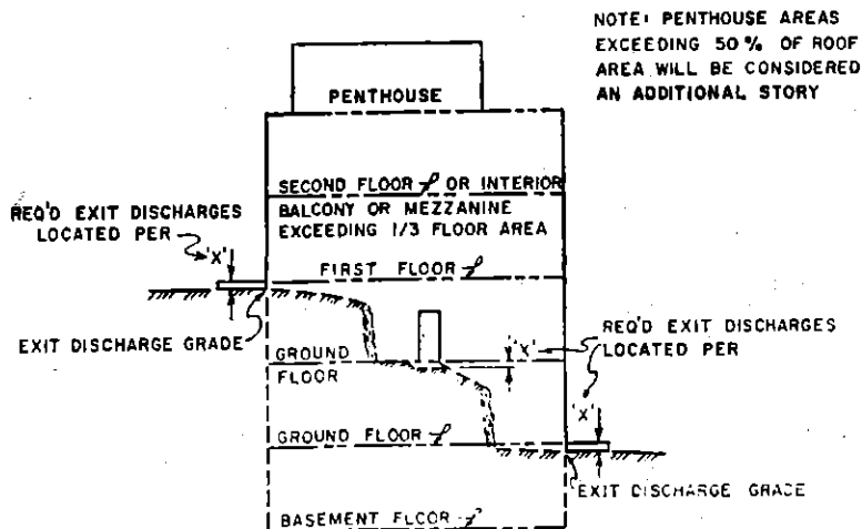
ILLUSTRATION SHOWING POSSIBLE 2 STORY CONDITION OR 3 STORY WITH PENTHOUSE NOTE: FOR ADDITIONAL VARIATIONS TO NO. OF STORIES SEE AND 502.03(4) ILLUSTRATION A-2
