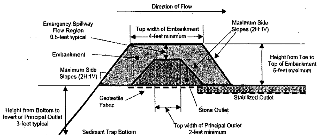
View A - A of Principal Outlet
