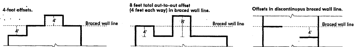
FIGURE 21.25-C PERMITTED OFFSETS
