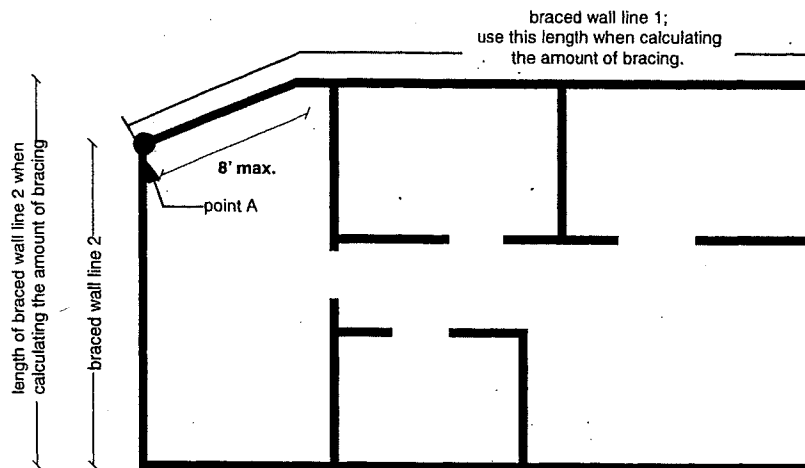
FIGURE 21.25-D ANGLED CORNERS
