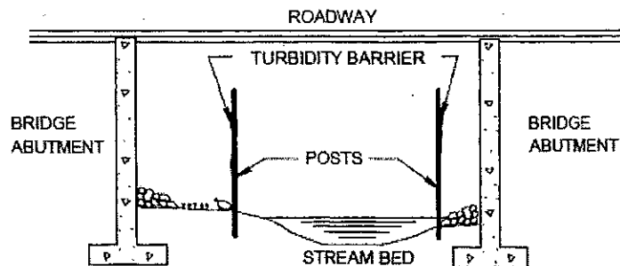
SECTION C-C
