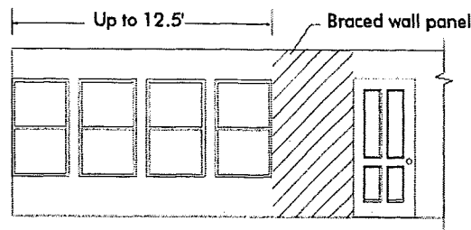
FIGURE 21.25-B PERMITTED BRACED WALL PANEL DISTANCES FROM ENDS OF A BRACED WALL LINE
