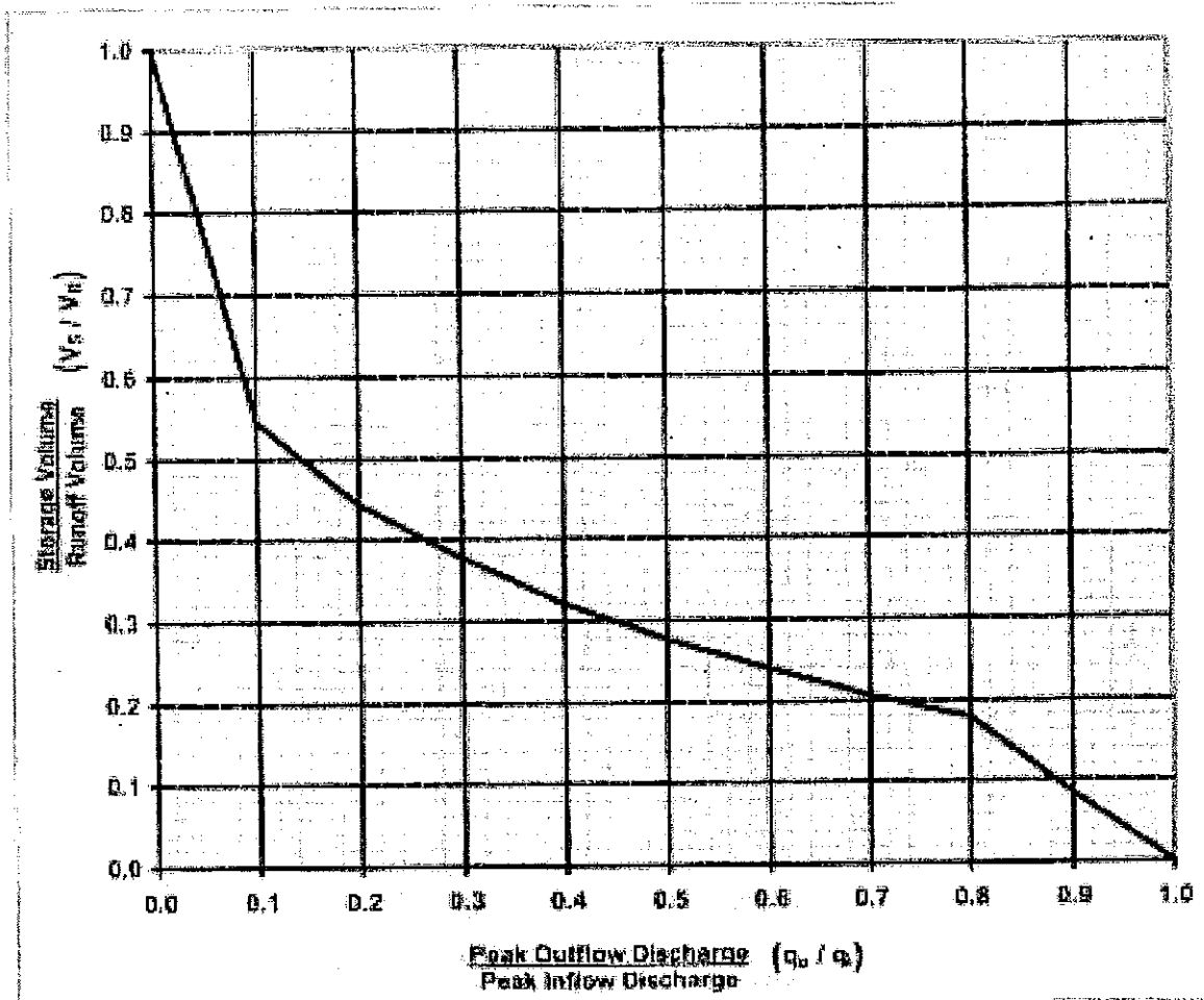
Figure 2 Approximate Detention Basin Routing for Type-II Storms
