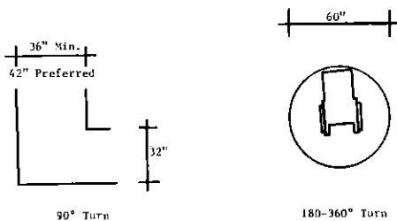
TURNING SPACE
