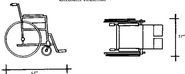
WHEELCHAIR DIMENSIONS
