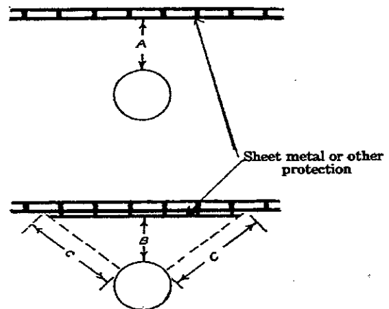
FIGURE 23.045-A CONSTRUCTION USING COMBUSTIBLE MATERIAL
