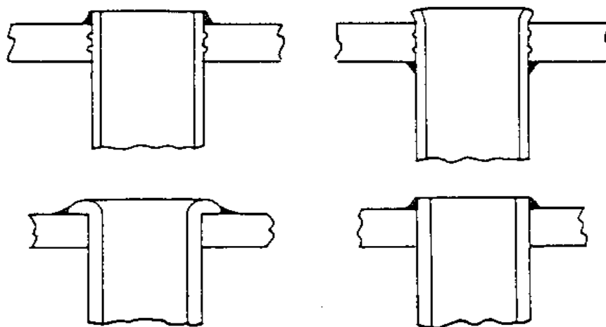
Figure 42.10-1 SEAL WELDING OF TUBES
