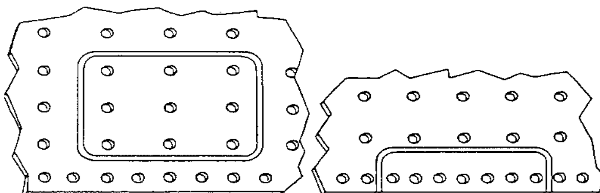
FLUSH PATCHES IN STAYED AREAS
