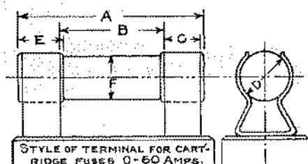
Form 1. CARTRIDGE FUSE—Ferrule Contact
