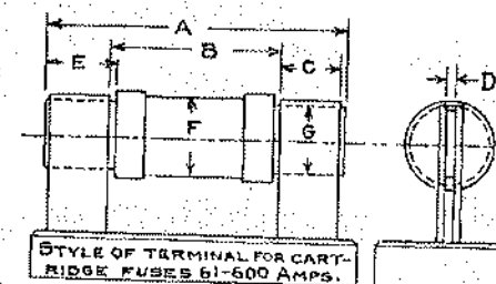
Form 2. CARTRIDGE FUSE—Knife Blade Contact
