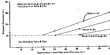
Figure 8-7(f) Wall Protection Using Material in Table 8-7(b).
