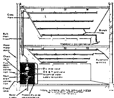
Figure 1-3(a) Dry-pipe system.
