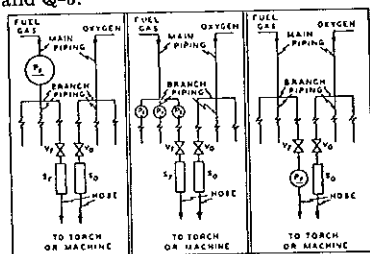
FIG. Q-1 FIG. Q-2 FIG. Q-3 P - Protective equipment in fuel gas piping V - Fuel gas station outlet valve W - Oxygen station outlet valve B - Backflow prevention device(s) at fuel gas station outlet S - Backflow prevention device(s) at oxygen station outlet
