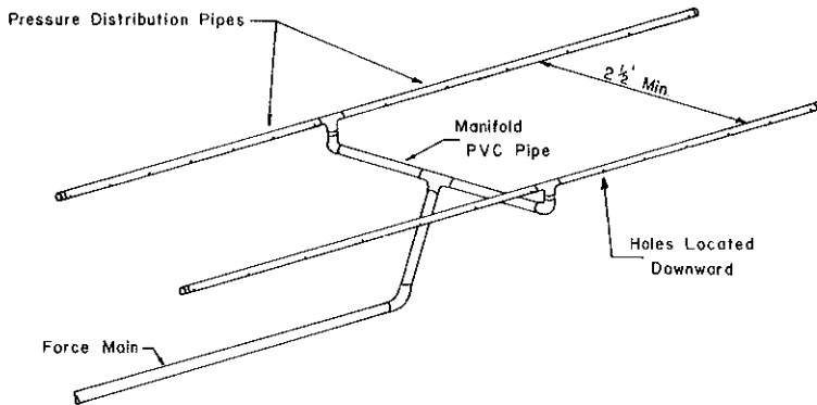
Bed Design Is Recommended Over Trenches
