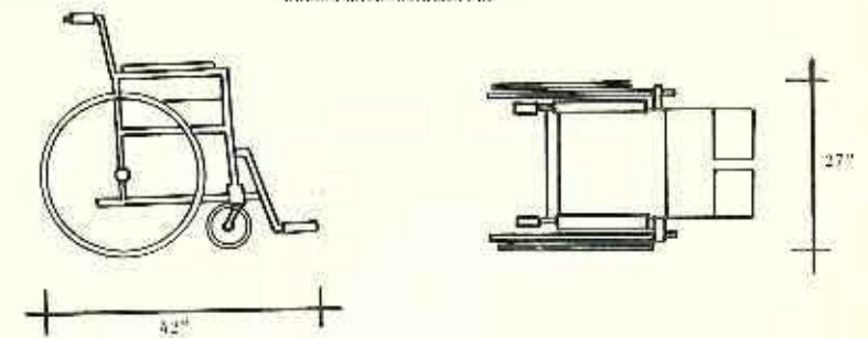
WHEELCHAIR DIMENSIONS
