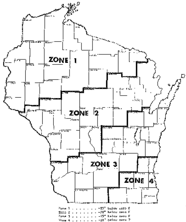
MAP OF WISCONSIN SHOWING DESIGN TEMPERATURE ZONES
