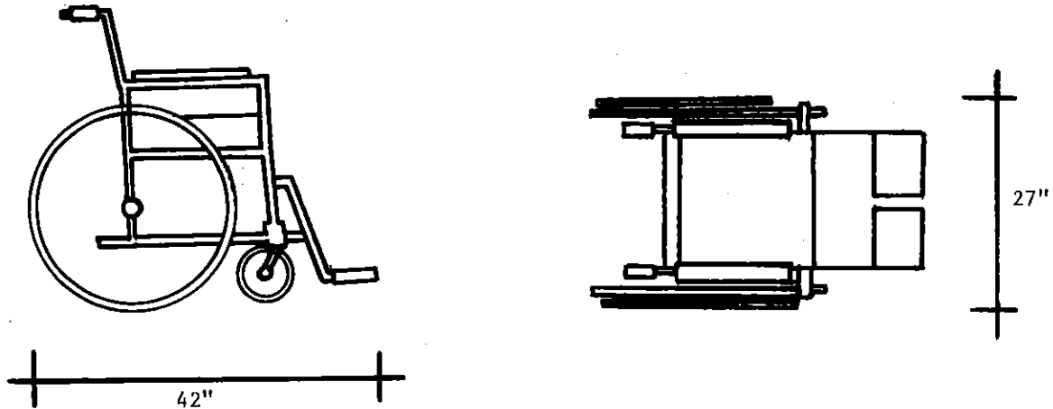
WHEELCHAIR DIMENSIONS
