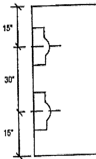
Figure A-84.20-2. Spacing between stall type urinals.
