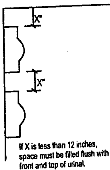
Figure A-84.20-4. Spacing between urinals.
