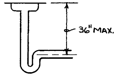
FLOOR DRAIN
