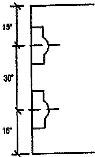
Figure A-84.20-2. Spacing between urinals.
