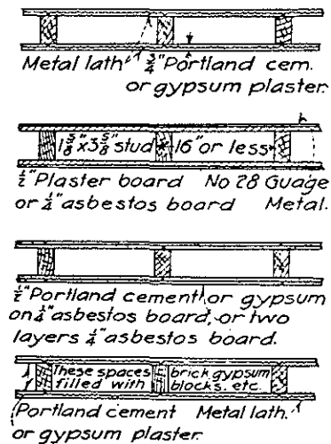
SEMI-FIREPROOF PARTITIONS
