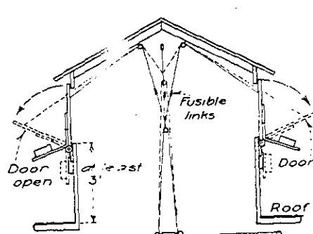
SECTION OF WOODEN VENTILATOR AUTOMATIC STAGE VENTILATOR
