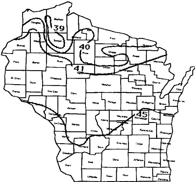
Mean Annual Temperature Contour Map
