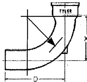
Radius of hub &amp; spigot fitting
