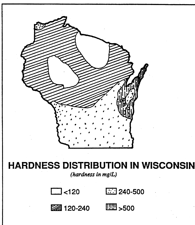
Figure 1-10: Hardness of Wisconsin's Groundwater
