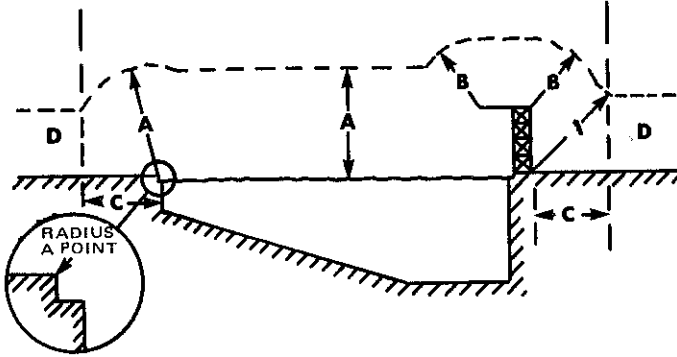
Figure PSC 114-234-2 SWIMMING POOL CLEARANCES
