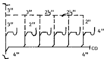
4" TRAP SERVING 4 WASHERS
