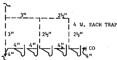
4" TRAP SERVING 4 WASHERS
