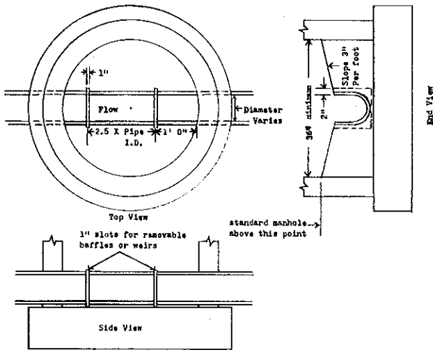
TYPICAL SAMPLING MANHOLE Section ILHR 82.04 (4) (i)
