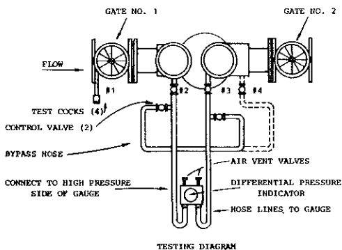
DIFFERENTIAL PRESSURE INDICATOR METHOD FOR REDUCED PRESSURE BACKFLOW PREVENTERS
