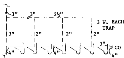
3" TRAP SERVING 3 WASHERS
