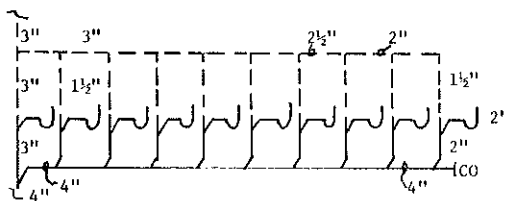
2" TRAP SERVING 2 WASHERS 20 TOTAL - 2 EACH TRAP
