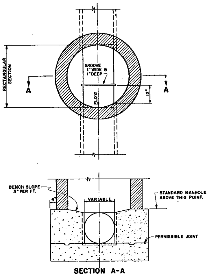
DETAIL OF SAMPLING MANHOLE
