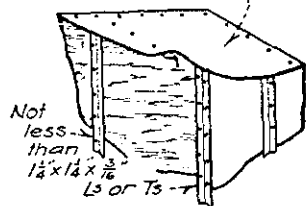
Typical Construction METAL OR ASBESTOS
