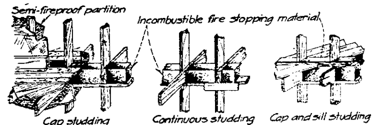
FIRE STOPPING
