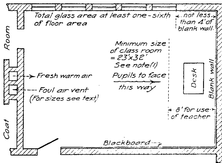
TYPICAL CLASS ROOM
