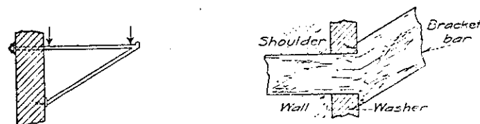
DETAIL OF WALL BEARING
