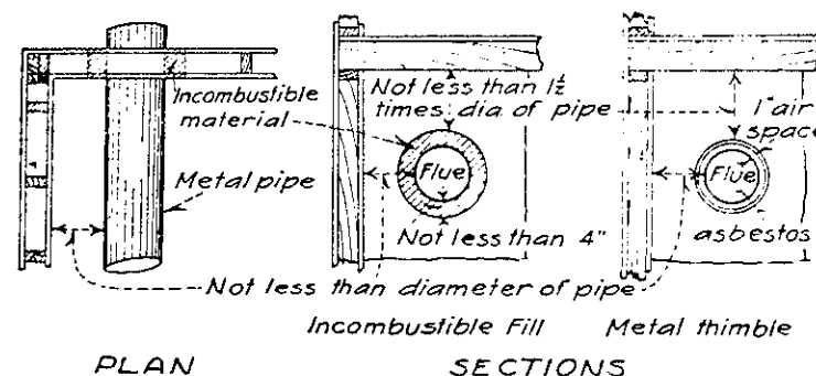
SECTIONS
