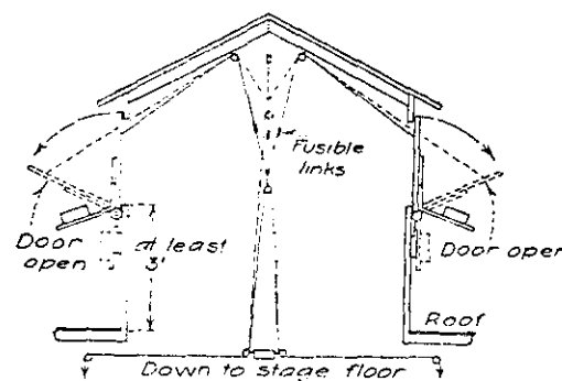
SECTION OF WOODEN VENTILATOR
