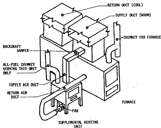
FIGURE 323.045-D
