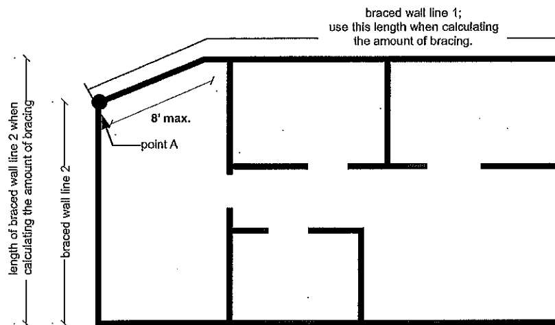
FIGURE 321.25-D ANGLED CORNERS
