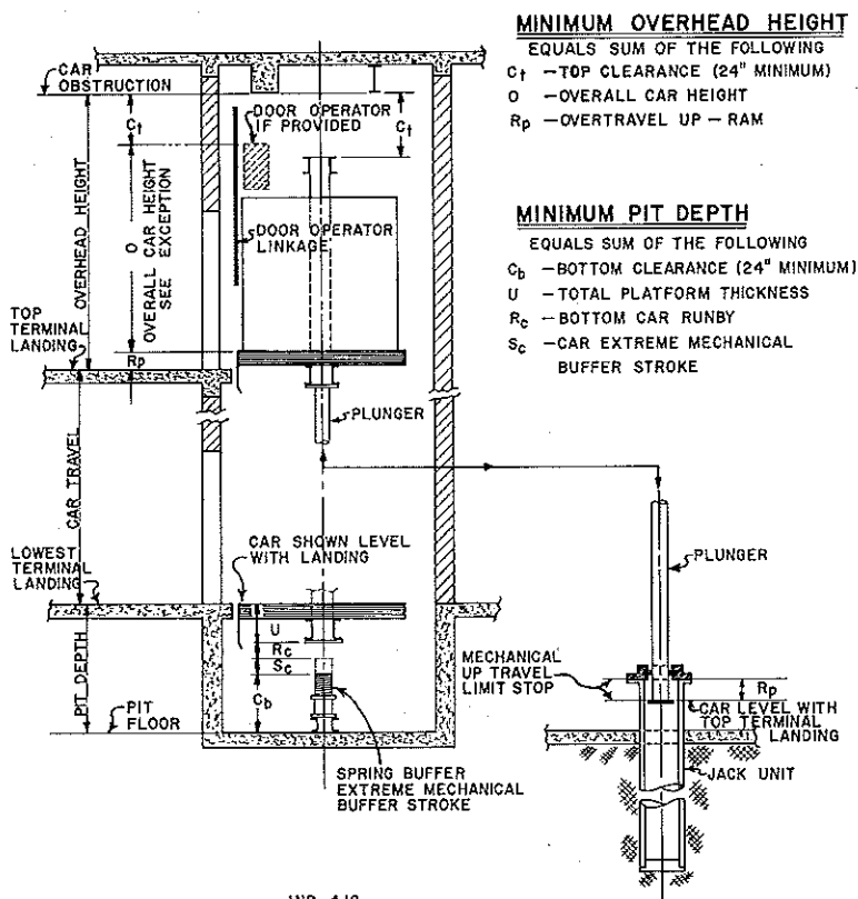
PIT DEPTH AND OVERHEAD HEIGHT FOR DIRECT ACTING PLUNGER HYDRAULIC ELEVATORS
