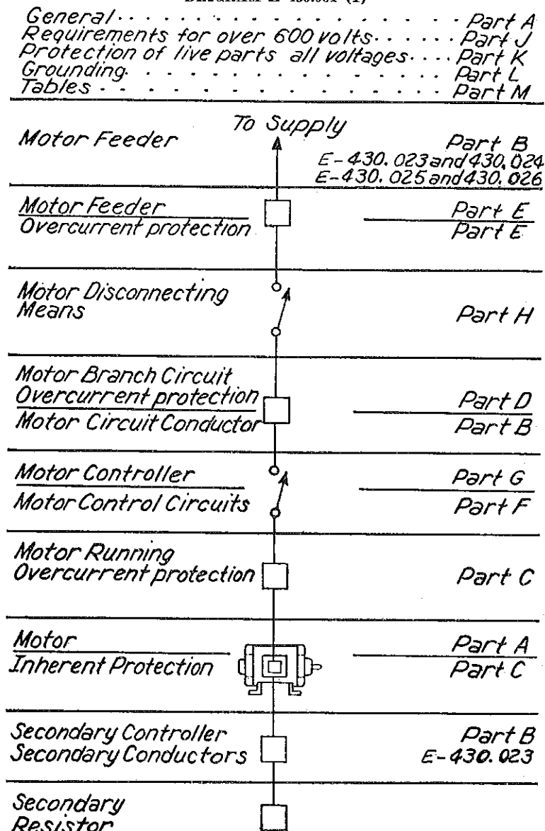
DIAGRAM E 430.001 (1)
