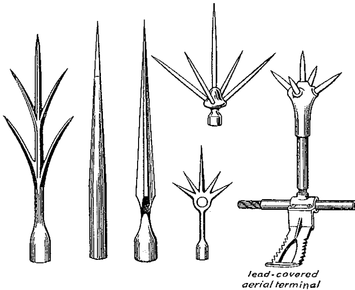
Air Terminals
