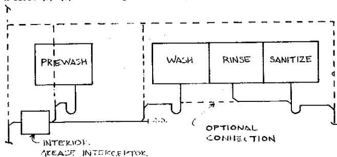
PREWASH AND 2-COMPARTMENT SCULLERY SINK
