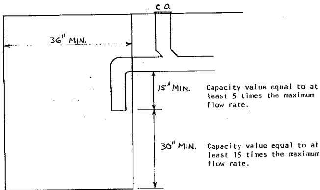
CAR WASH INTERCEPTOR WITH CAST IRON INVERT INSIDE OF BASIN
