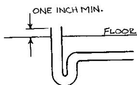
STANDPIPE IN FLOOR
