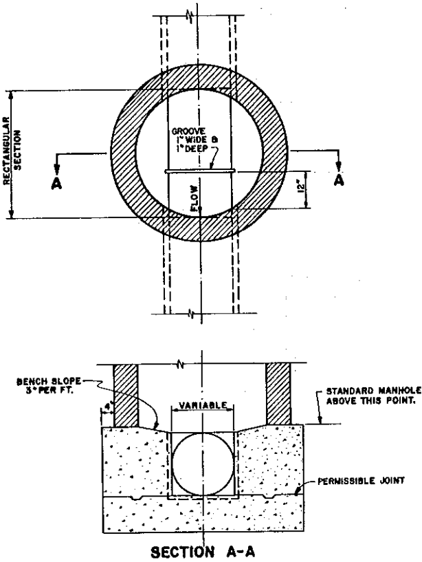
SECTION A-A DETAIL OF SAMPLING MANHOLE
