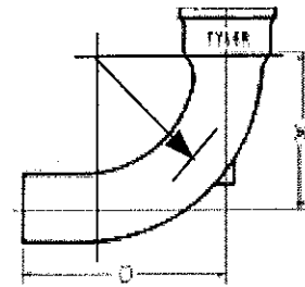
Radius of hub &amp; spigot fitting
