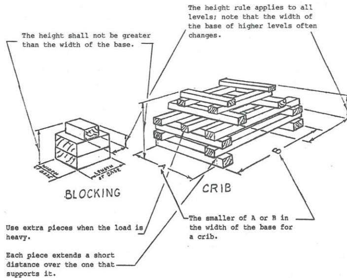
FIGURE 34.23-1 SYSTEMS OF BLOCKS
