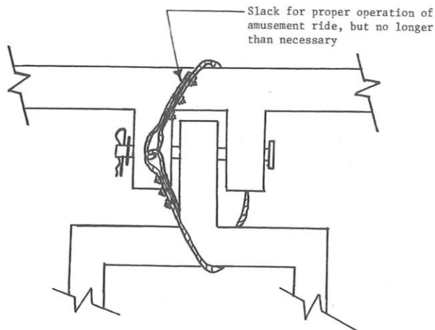
FIGURE 34.38-2 SAFETY CABLES
