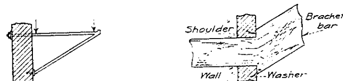
DETAIL OF WALL BEARING
