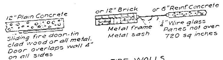
STANDARD FIRE WALLS
